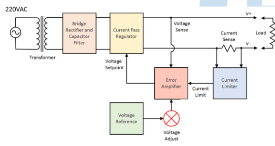
Gambar 5. Diagram blok power supply
