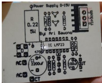
Gambar 8. Hasil PCB regulator LM723
